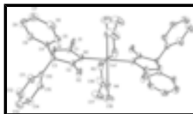
Fig. 1. The molecular structure of the title complex showing displacement ellipsoids drawn at the 30% probability level. H-atom are omitted for clarity. Unlabelled atoms are related to the labelled atoms by the symmetry operation 1-x, 1-y, -z.
